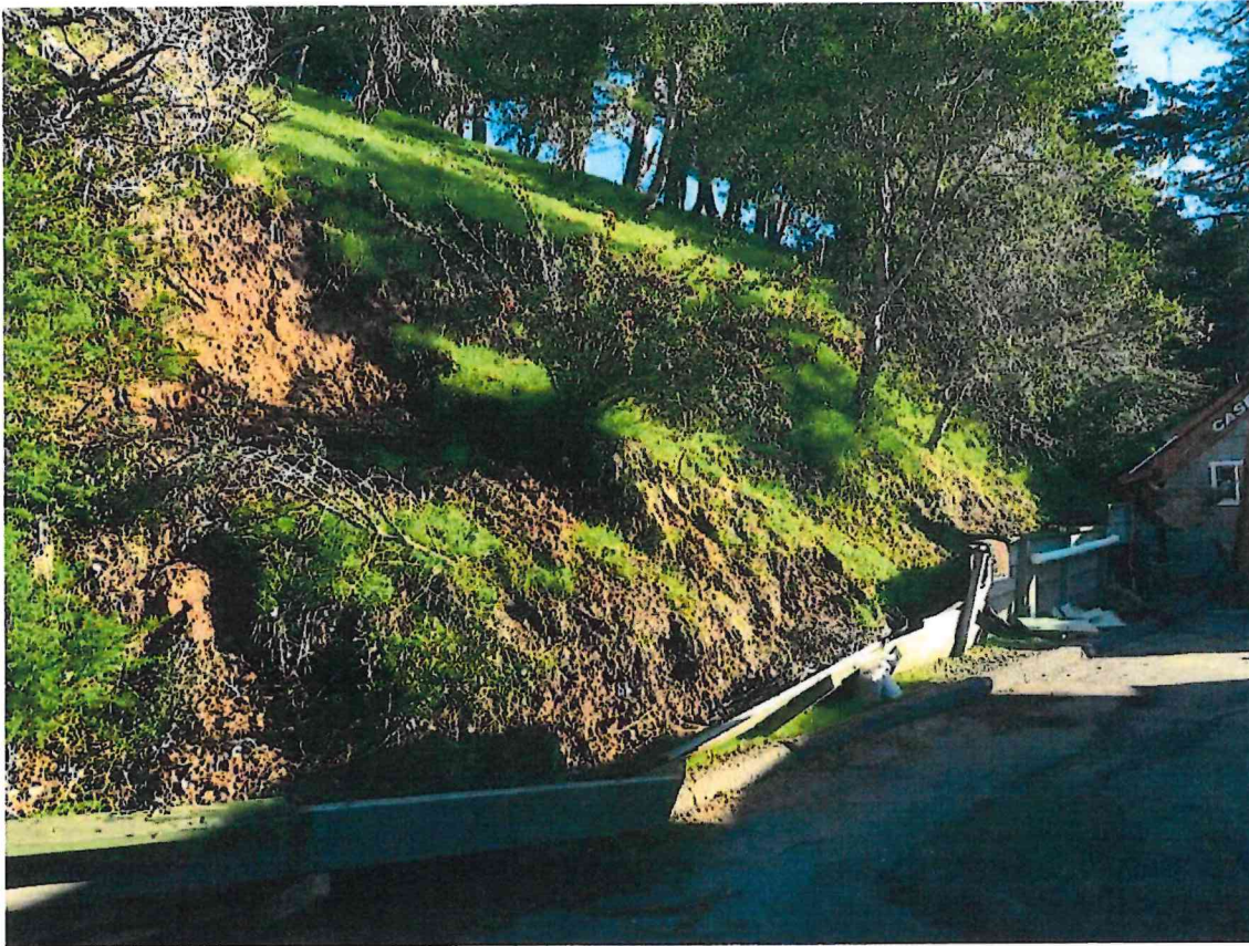
Figure 4: View northeast of failure of cut slope. Note proximity of building in back to cut slope and failure of wood wall. Trench T-1 was excavated near the building, Trench T-2 was excavated in the slide, and Trench T-3 was excavated just left of the sight of the picture.
