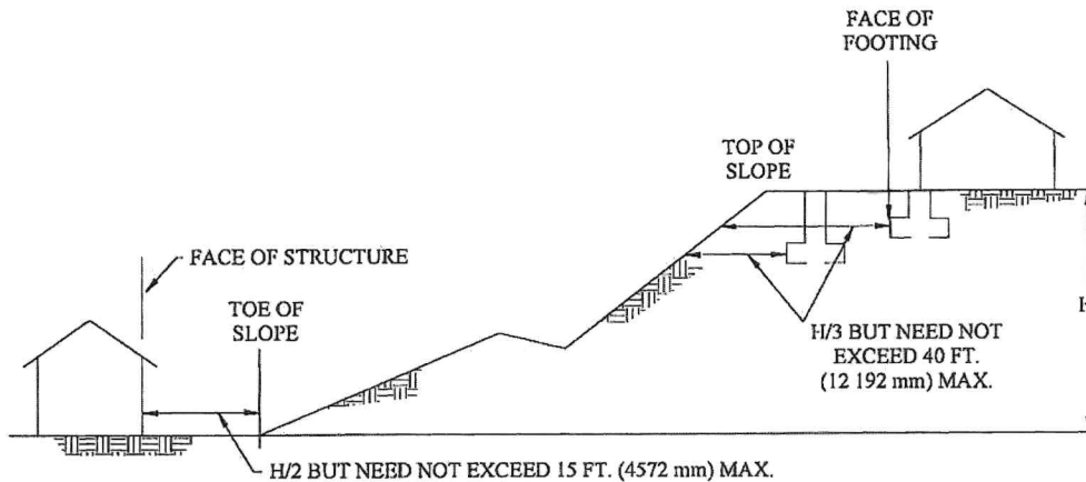
Figure 2: Building Setback Distance
